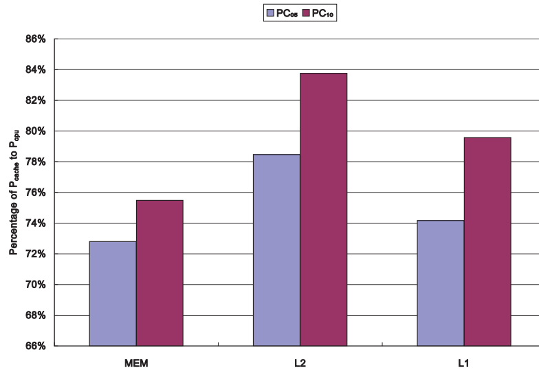
Figure 3.8: The impact of the power of cache on the power of CPU.
