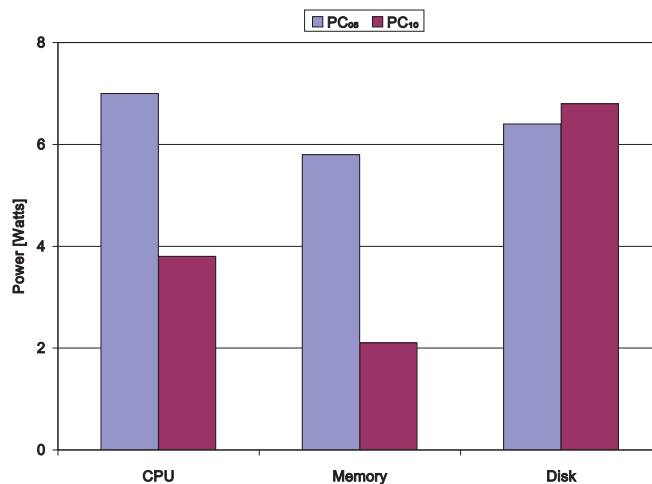
Figure 3.4: Power dissipation comparison of the main component.
