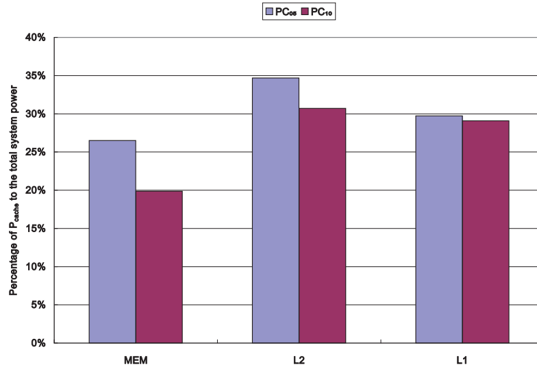
Figure 3.9: The impact of the power of cache on the power of the whole computer system.
