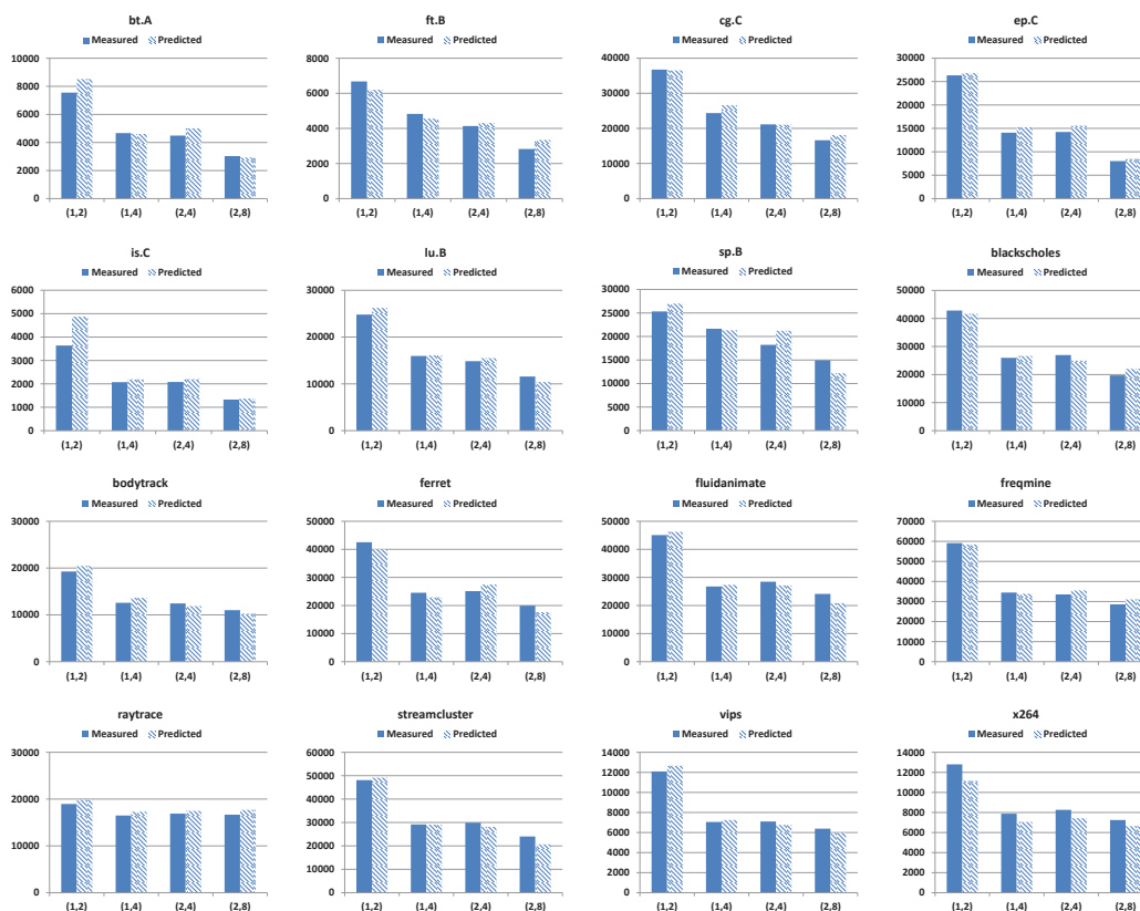
Figure 7.7: Measured energy consumption vs. predicted energy consumption. The unit is in Joule. X-axis represents one configuration. For example, (1,2) stands for one processor and totally two threads are used.
