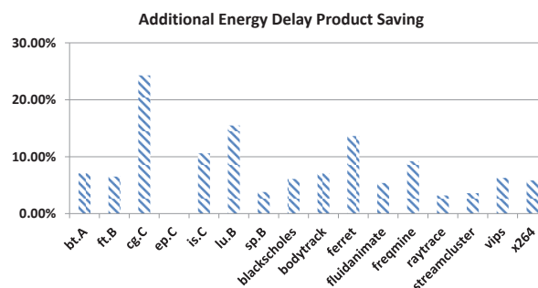
Figure 7.8: Additional EDP using run-time DVFS when the optimal configuration generated from the first step is used. The results are compared to the setting that uses maximum frequency only.
