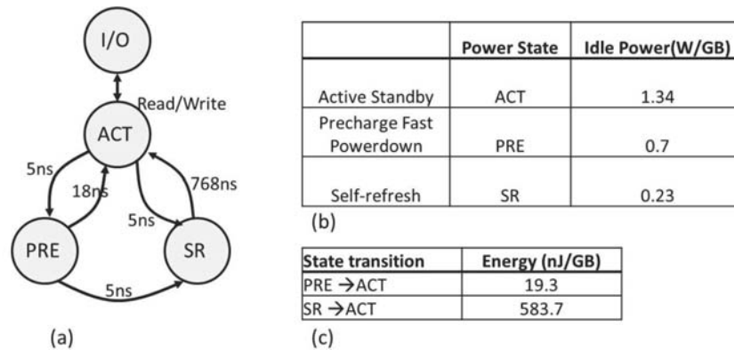
Figure 2.1: Memory System Architecture. (figure courtesy of [141])
